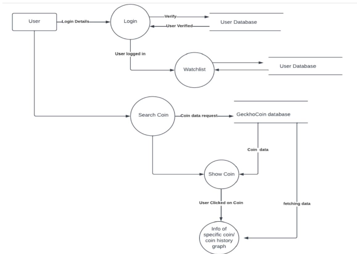
Fig.2. DFD for Proposed Architecture
