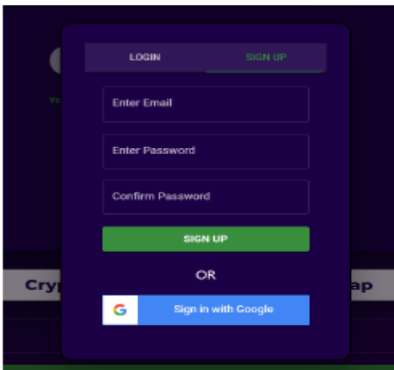
Fig.3. Login/Logout Interface
